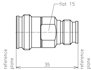
all dimensions in millimeter
