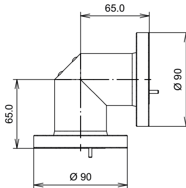
90° Elbow BN 938520
